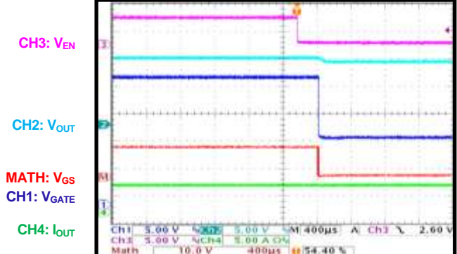
Shutdown through EN (for Smart Diode)
