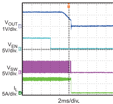
Shutdown through V_{EN} I_{OUT} = 6A
