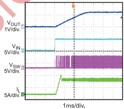
Start-Up through V_{EN} I_{OUT} = 6A
