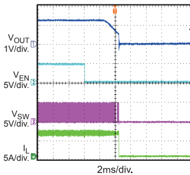
Shutdown through V_{EN} I_{OUT} = 6A
