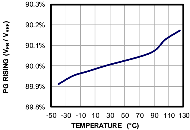
PG Rising Threshold (V FB Rising) vs. Temperature
