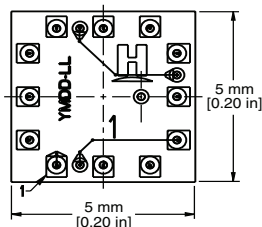
FIGURE 2. PAD FUNCTIONS
