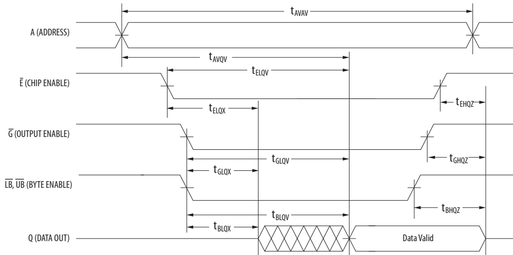
Figure 9 – Read Cycle 2
