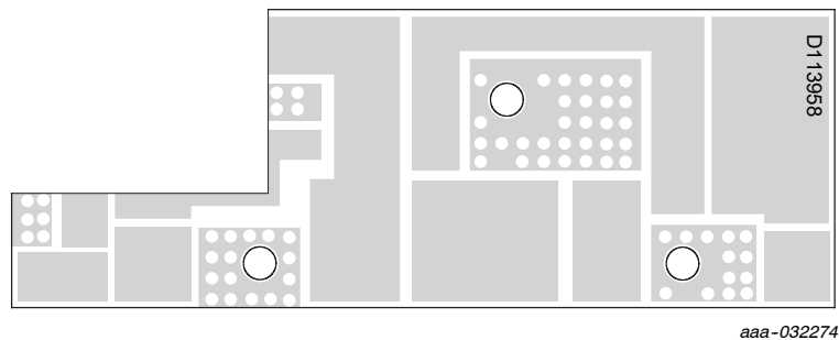
Figure 4. MRF101AN Compact Reference Circuit Board
