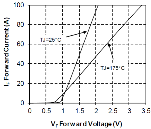
Figure 18 • Forward Characteristics
