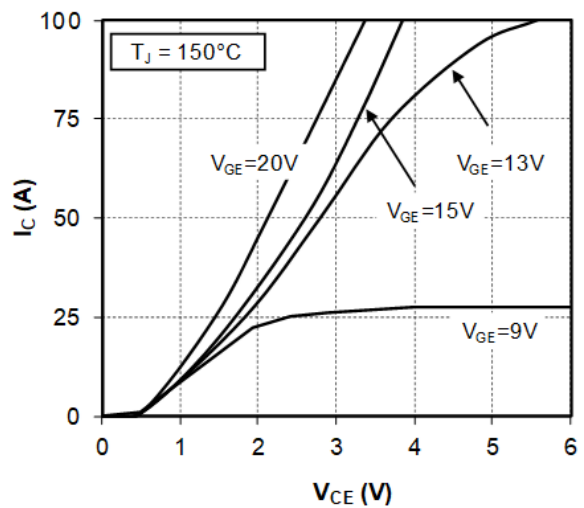
Figure 1-3. Output Characteristics
