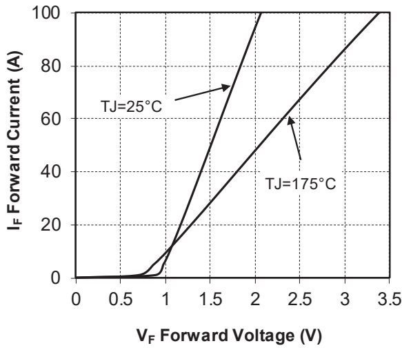
Figure 1-9. Forward Characteristics
