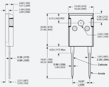
TO-247 2-Lead
