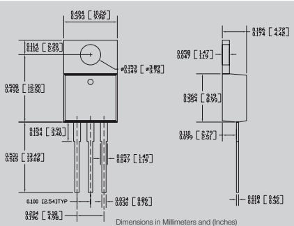
TO-220 3-Lead
