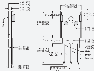
TO-247 3-Lead
