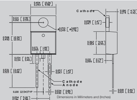
TO-220 2-Lead
