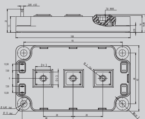
SP6-Three Outputs
