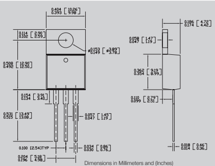
TO-220 3-Lead
