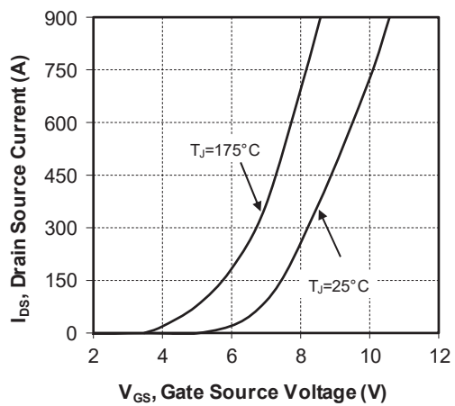
Figure 1-5. Transfer Characteristics
