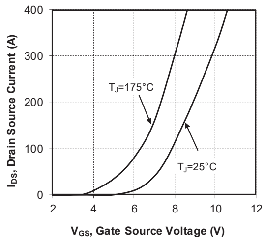
Figure 1-5. Transfer Characteristics
