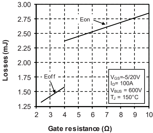
Figure 1-6. Switching Energy vs. Rg
