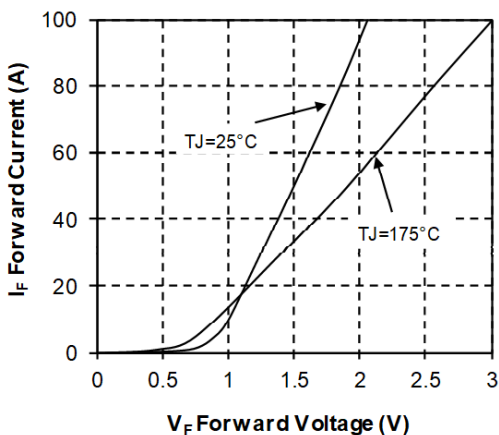
Figure 19 • Forward Characteristics
