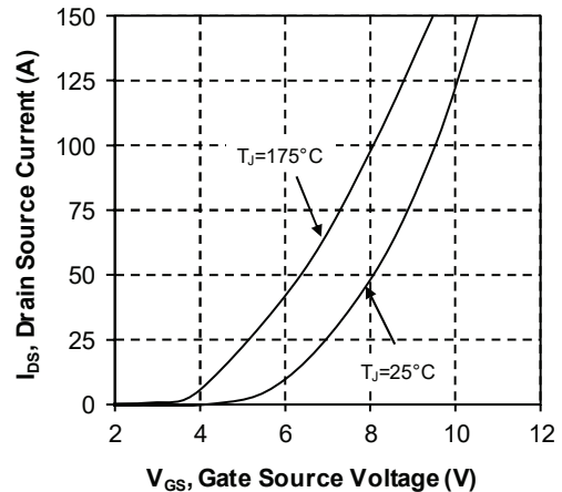
Figure 1-5. Transfer Characteristics
