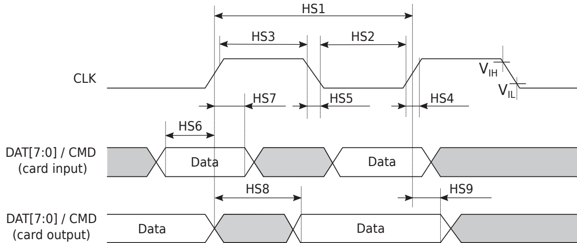
Figure 3-3 MSDC Timing Diagram (High Speed mode)
