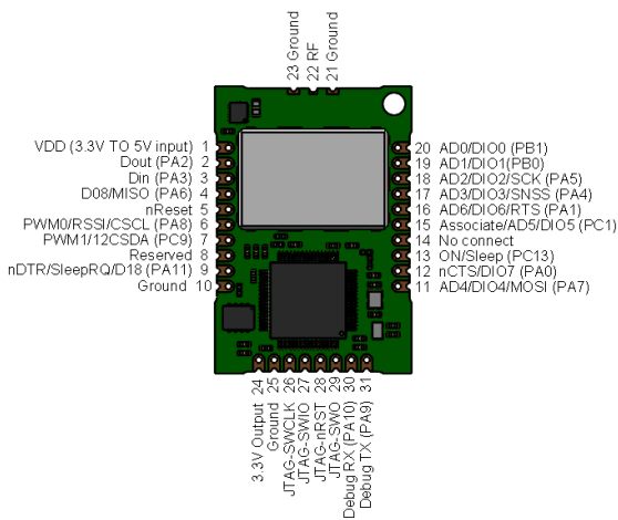
MTDOT-868-M1-TRC MTDOT-915-M1-TRC
