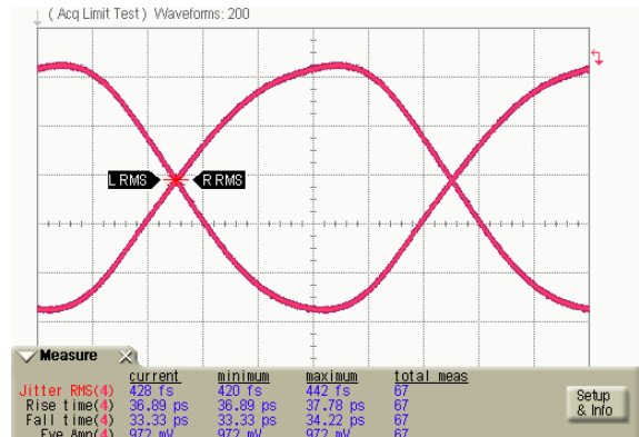
Divide-by-2 Output (Input: 10 GHz; Output: 5 GHz)
