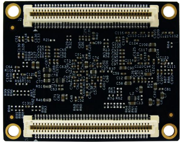
Figure 1-2 MYC-C335X-GW Bottom-view
