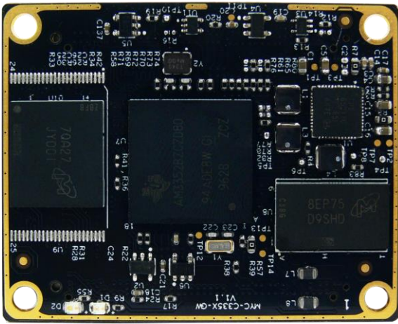
Figure 1-1 MYC-C335X-GW Top-view
