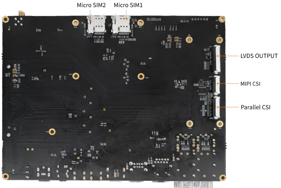
Figure 1-5 MYD-JX8MMA7 Development Board Bottom-view
