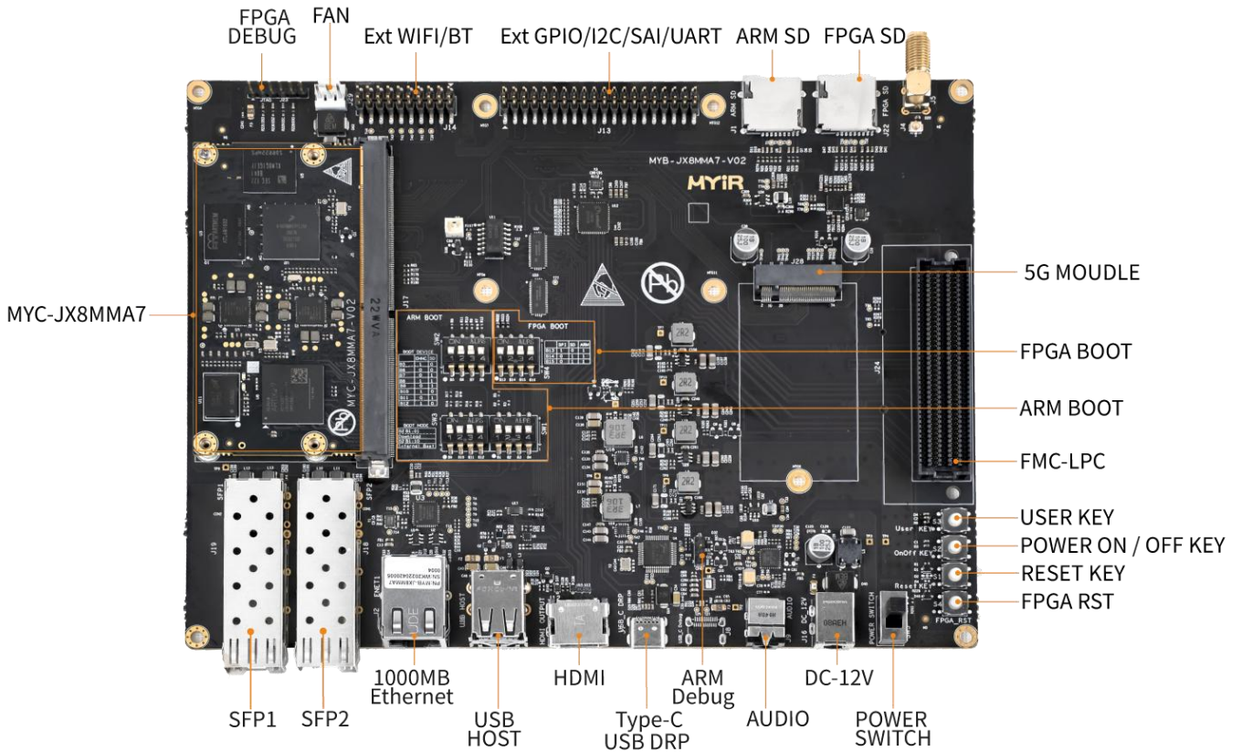
Figure 1-4 MYD-JX8MMA7 Development Board Top-view
