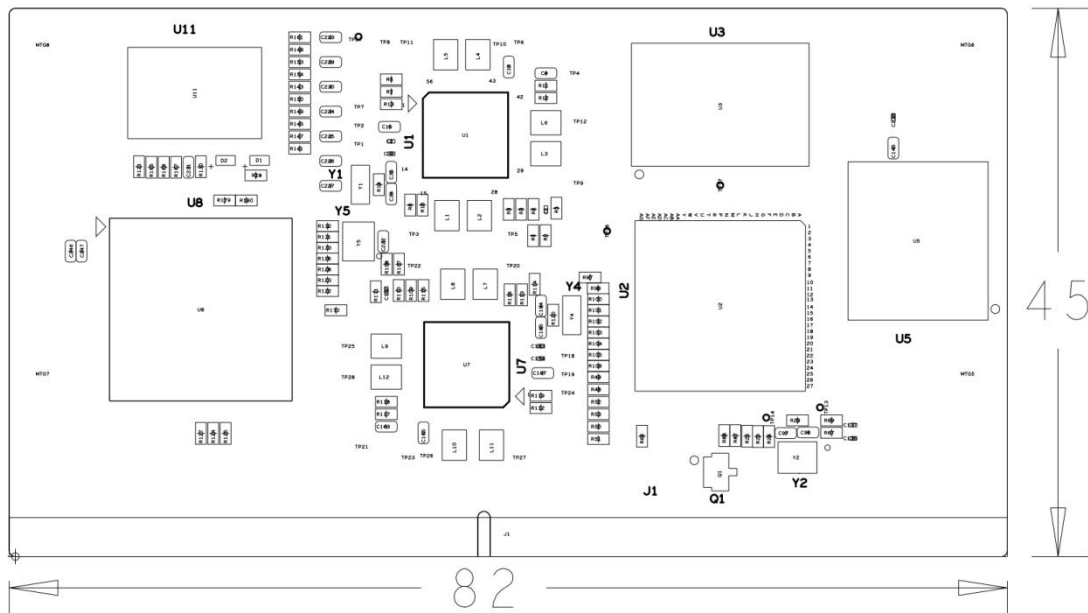
Figure 1-7 MYC-JX8MMA7 Dimensions Chart (Unit: mm)
