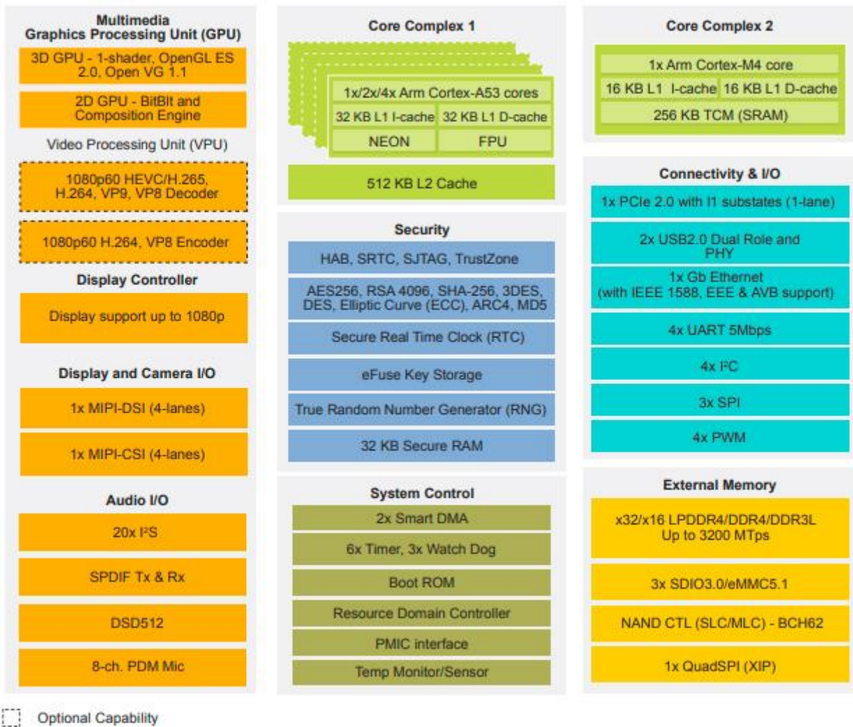
Figure 1-6 i.MX 8M Mini Processors Family Block Diagram
