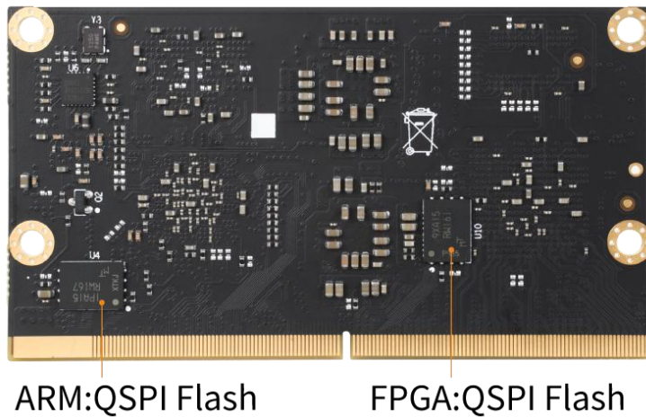
Figure 1-3 MYC-JX8MMA7 CPU Module Bottom-view
