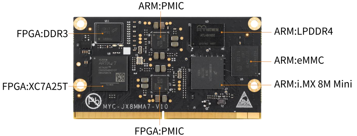
Figure 1-2 MYC-JX8MMA7 CPU Module Top-view
