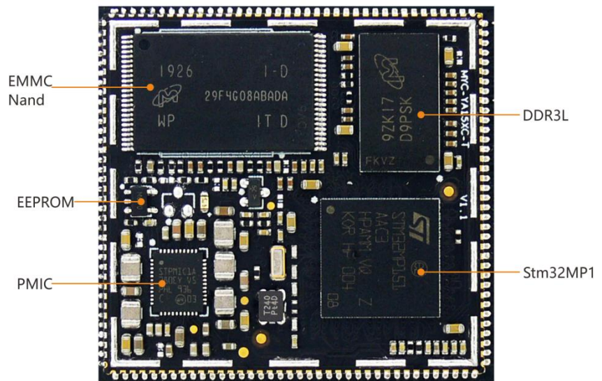
MYC-YA15XC-T CPU Module
