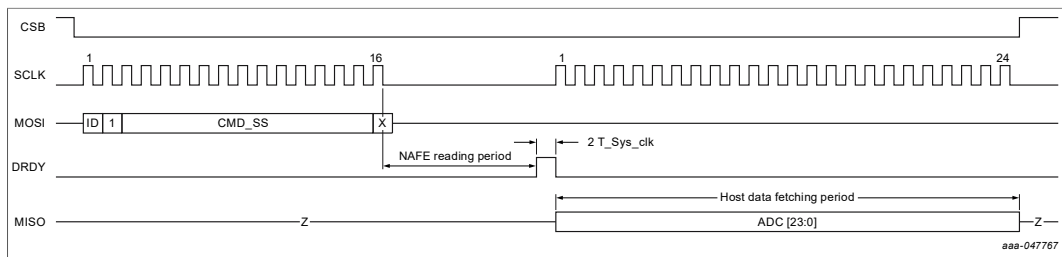
Figure 20. CMD_SS timing diagram with CSB low
