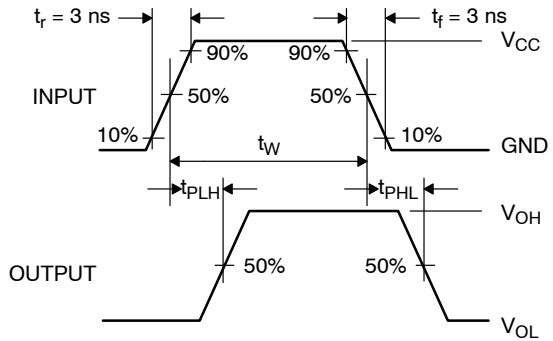
Figure 7. AC Waveforms
