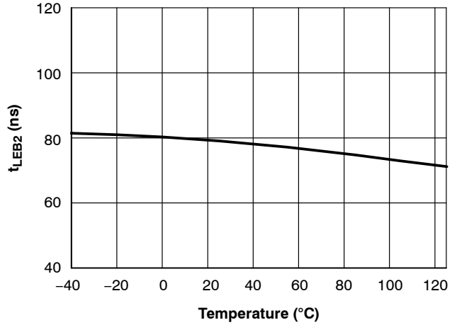
Figure 17. t_{LEB2} vs. Junction Temperature
