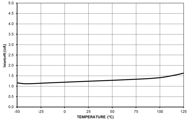
Figure 6. Off-state Leakage Current from HV Pin I_{start(off)}
