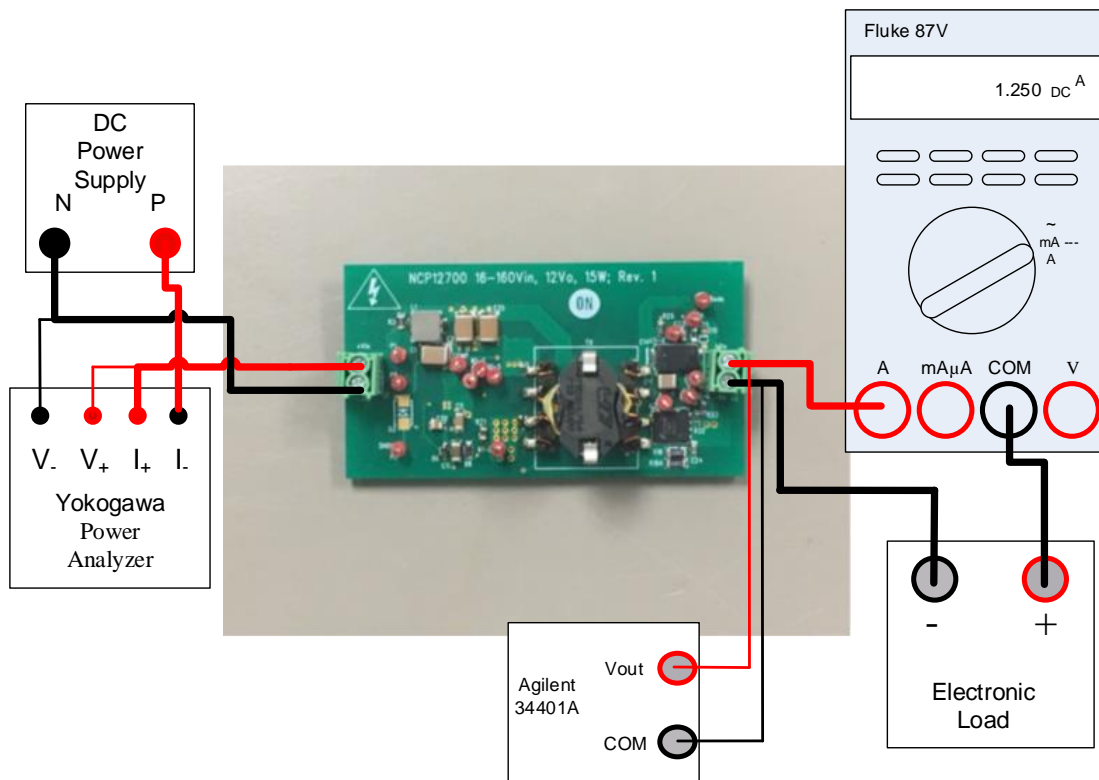
Figure 1: Test Setup
