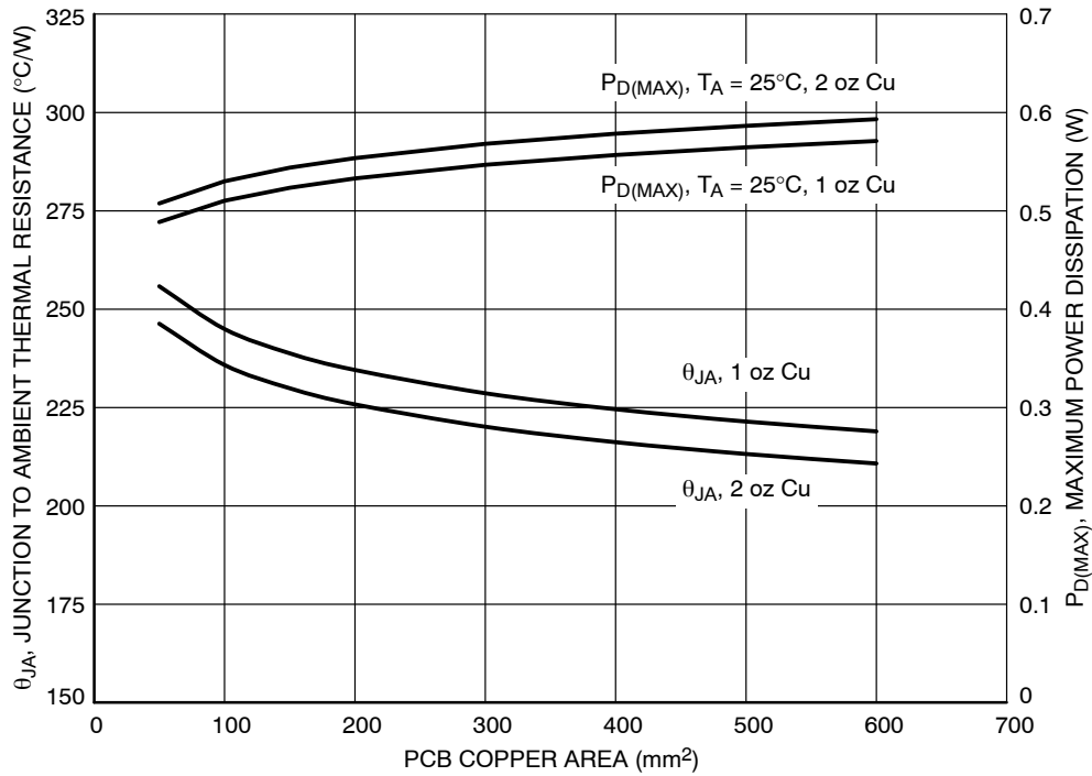
Figure 52. \theta_{JA} and P_{D(\text{MAX})} vs. Copper Area (SOT23-5L)
