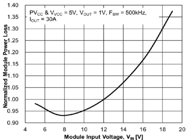
Figure 8. Power Loss vs. Input Voltage
