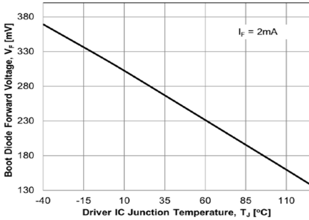
Figure 21. Body Diode Forward Voltage vs. Temperature
