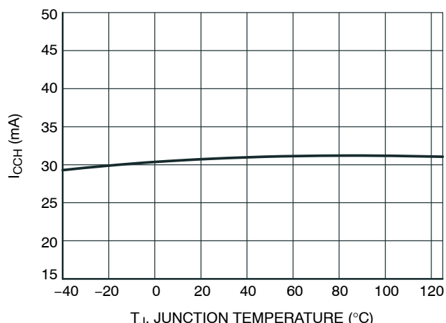
Figure 49. CCH Current to VCCL Pin, V_{CCH} = 8.0 V, V_{CCL} = 4.0 V
