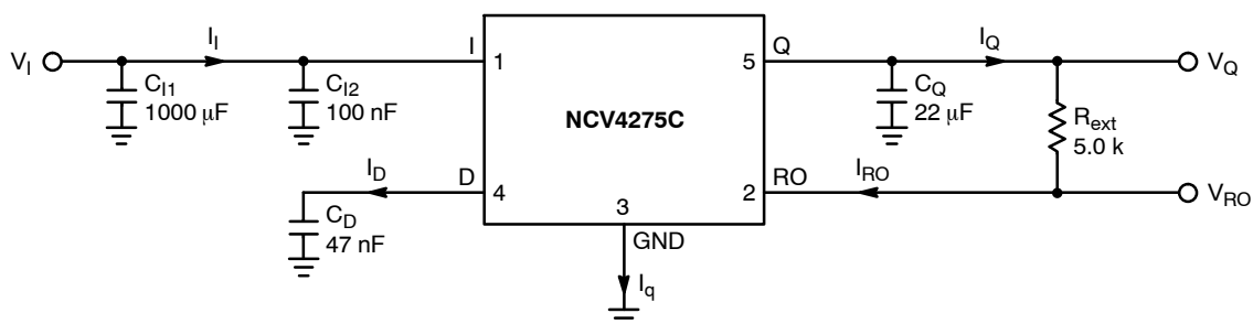
Figure 21. Test Circuit
