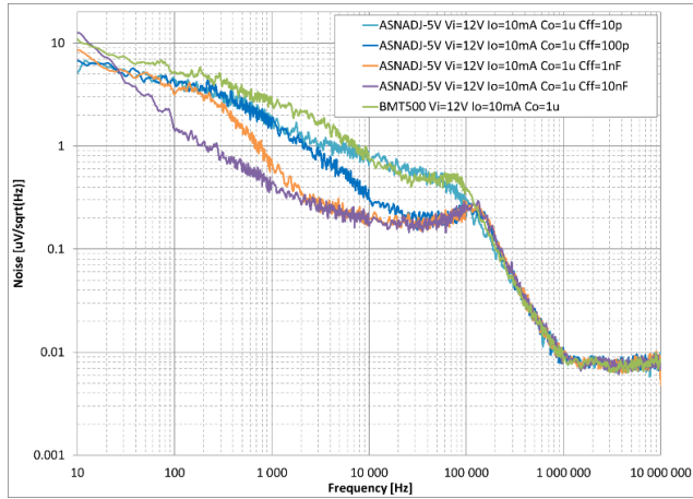
Figure 37. Noise – ADJ-set-5.0 V with Different C_{FF} and FIX – 5.0 V
