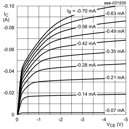
Fig. 5. NHDTA114EU: Collector current as a function of collector-emitter voltage; typical values
