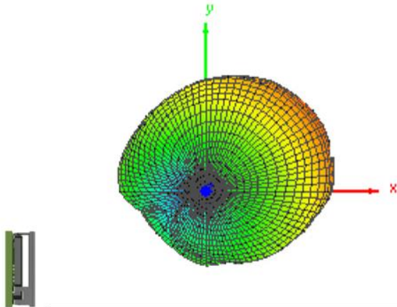
Theta = 0, Phi = 0
