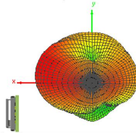
Theta = 180, Phi = 0
