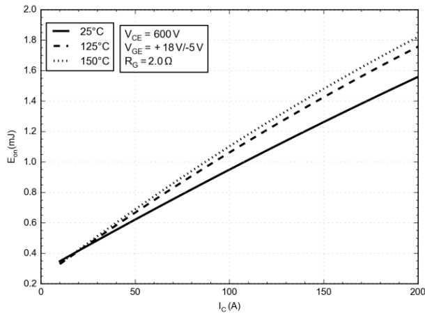
Figure 12. Typical Switching Loss E_{ON} vs. I_C
