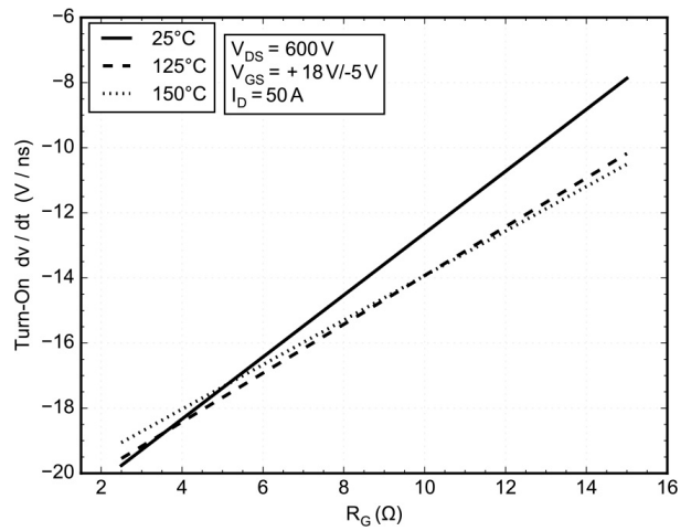
Figure 26. dv/dt ON vs. RG
