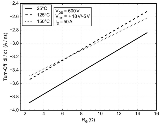
Figure 24. di/dt OFF vs. RG
