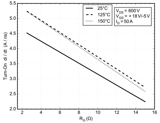
Figure 22. di/dt ON vs. RG
