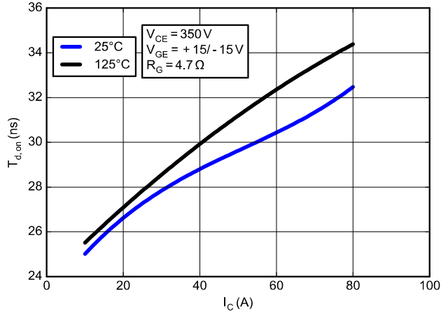
Figure 28. Typical On Switching Times vs. IC
