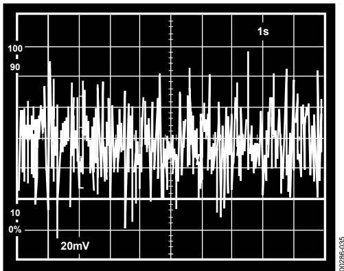
Figure 36. Input Voltage Noise @ \pm 15\text{ V} ( 20\text{ nV/div} )
