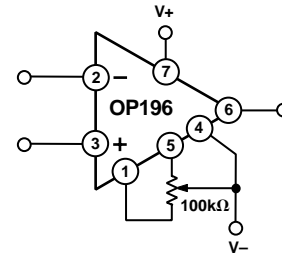
Figure 3. Offset Nulling Circuit
