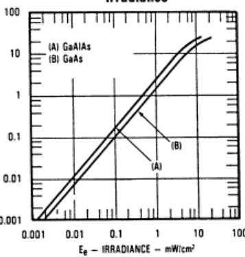
On-State Collector Current vs Irradiance
