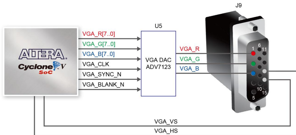
Figure 3-20 VGA Connections between FPGA and VGA
