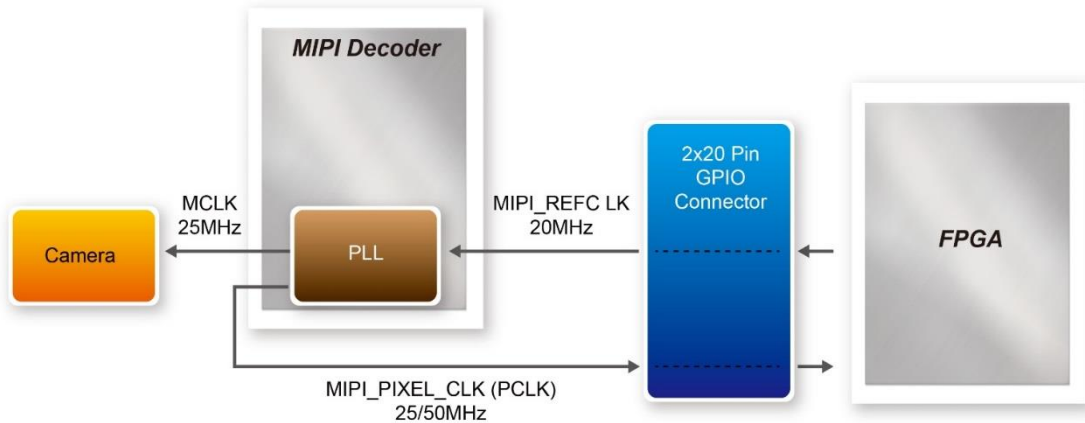
Figure 3-5 Simple Clock Tree of the D8M Board
