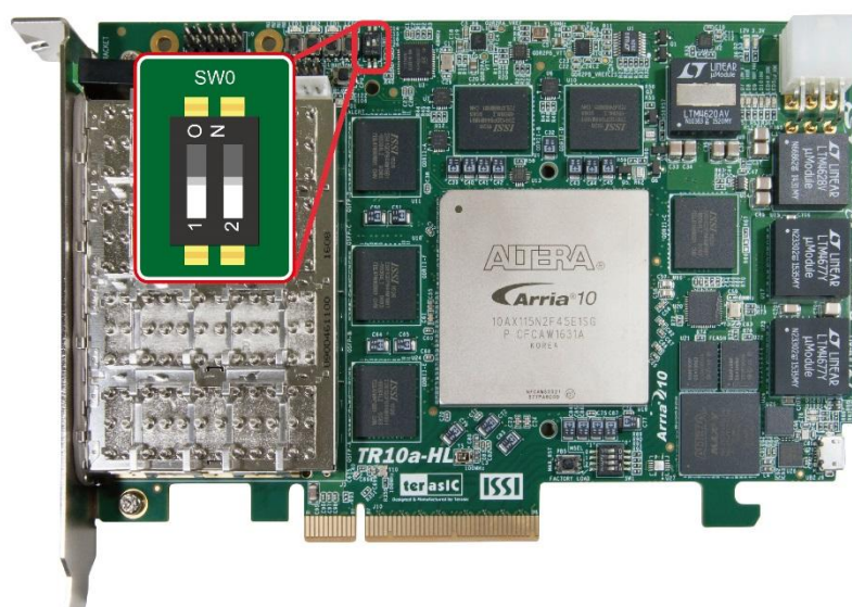
Figure 2-6 2 Dip switches
