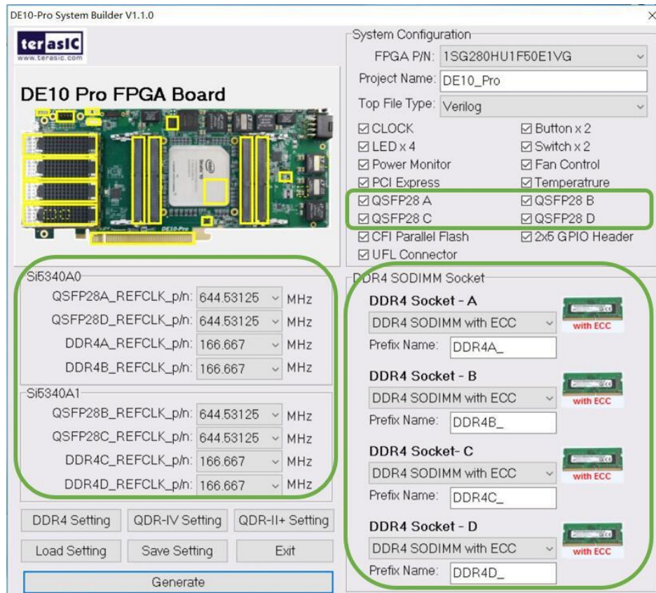
Figure 3-7 External programmable oscillators
