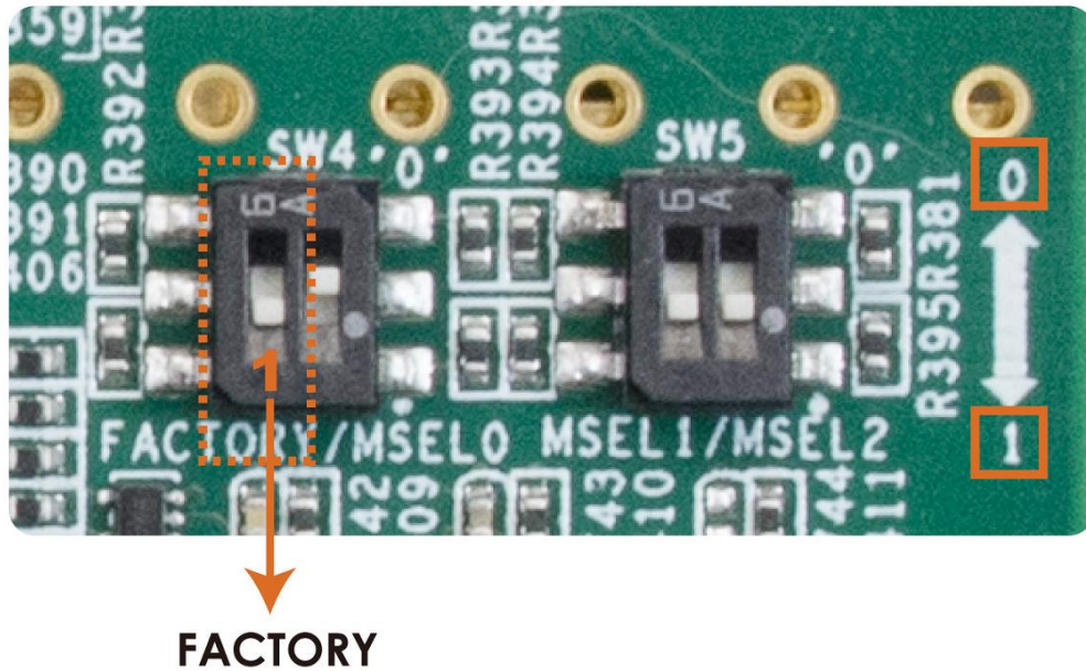
Figure 2-4 FACTORY position of slide switch SW4 for Image Select – Factory Image Load
