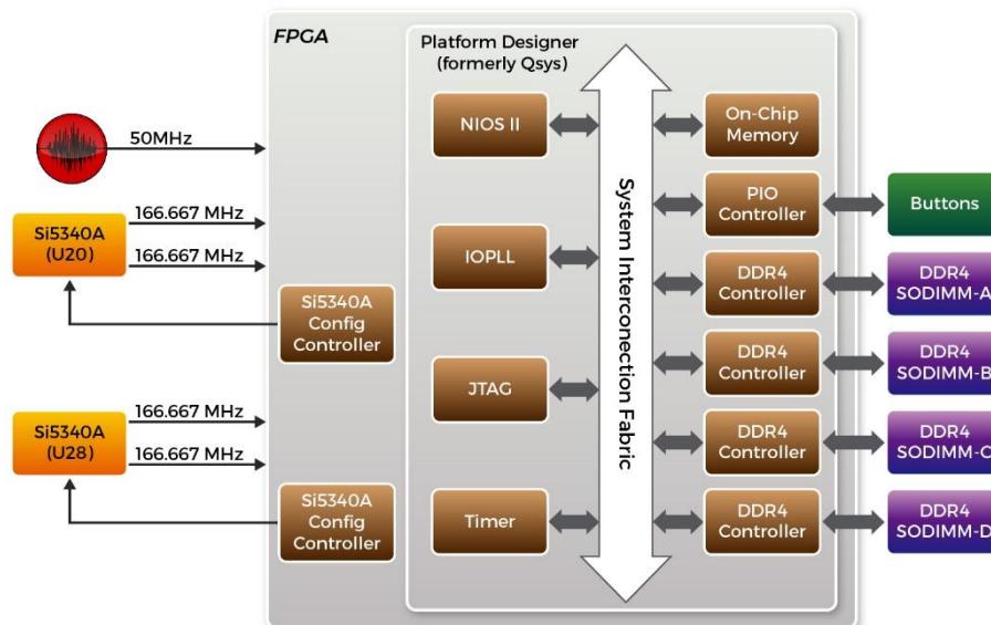
Figure 6-2 Block diagram of the DDR4 Basic Demonstration
