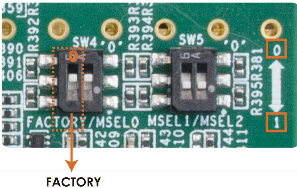
Figure 2-5 FACTORY position of slide switch SW4 for Image Select – User Image Load
