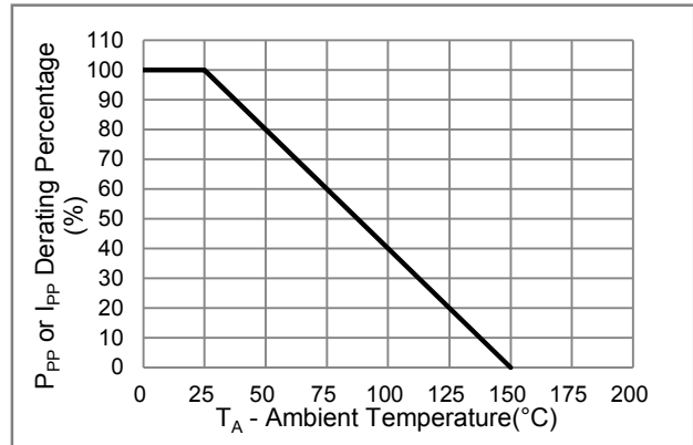
Fig.2 Derating Curve
