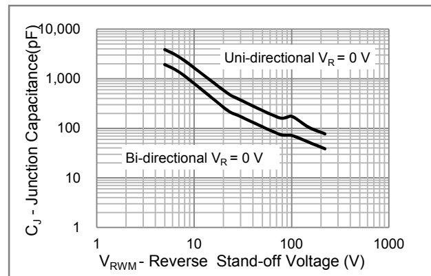
Fig.4 Typical Capacitance
