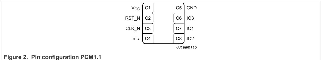
Figure 2. Pin configuration PCM1.1
