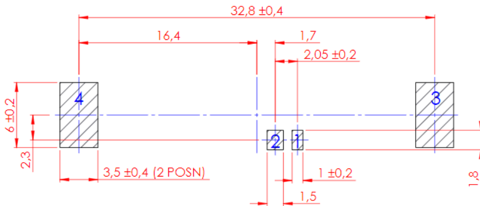
FOOTPRINT PCB
