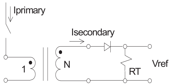
APPLICATION CIRCUIT
