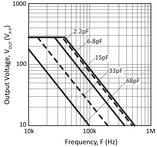
Figure 10: Slew Rate
